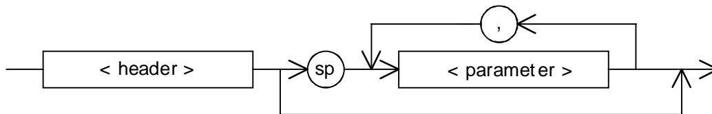
Fig. 1: Syntax of a program message unit
